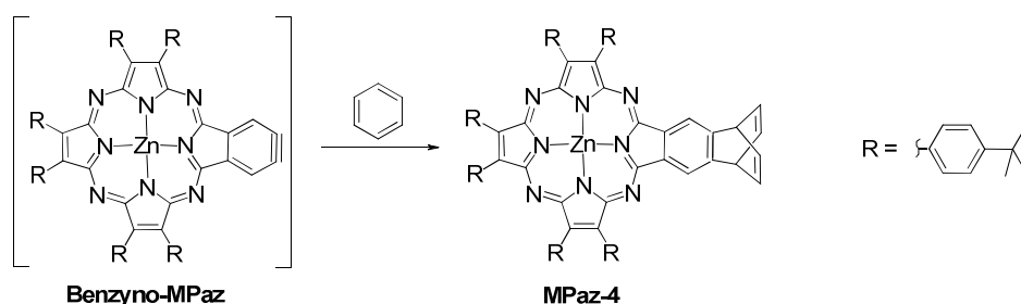
Scheme 9. Reaction of Benzyno-MPaz with benzene.
